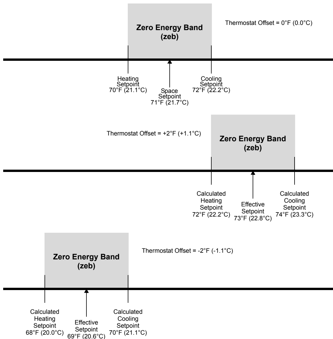
Figure 5: Setpoint Adjustment
