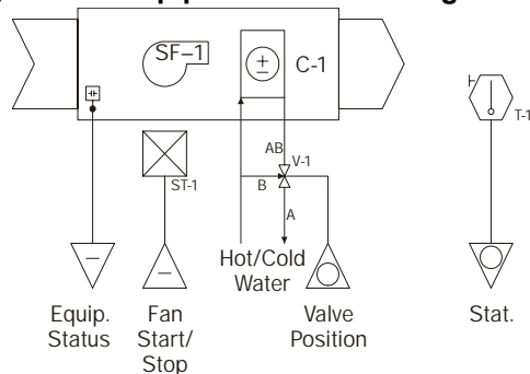
Figure 1: Two-pipe FCU with Analog Valve
