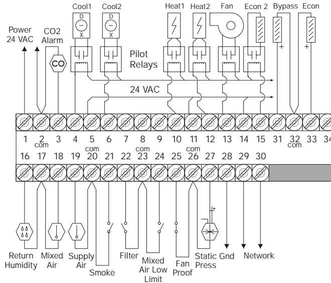
Figure 2: MPU-1 Terminal Connections
